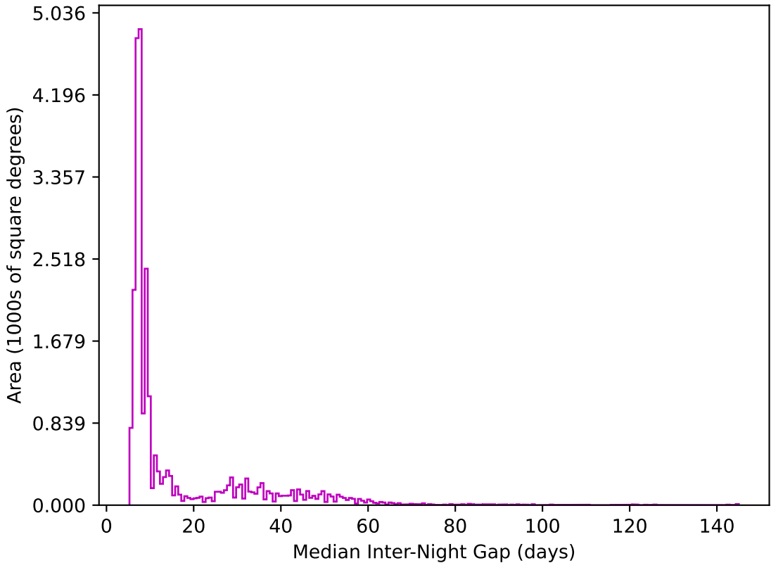
ddf_loaded_fl15_v3.4_10yrs All sky z band: Median Inter-Night Gap
