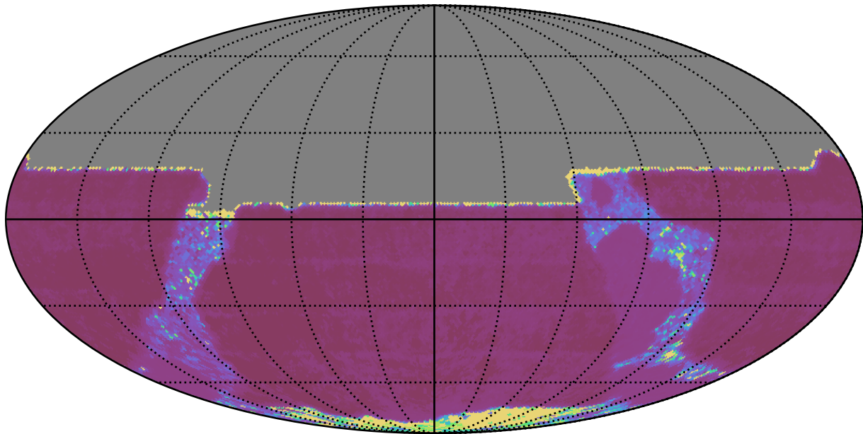
ddf_loaded_fl15_v3.4_10yrs All sky y band: Median Inter-Night Gap
