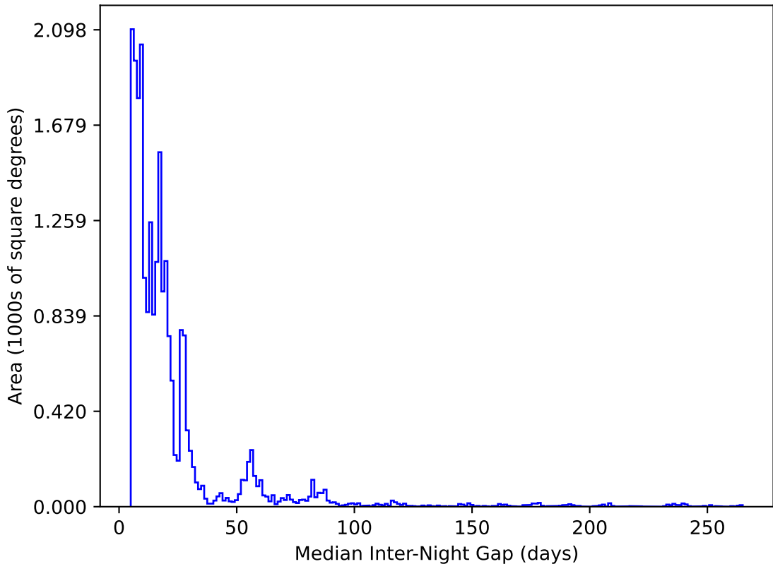
ddf_loaded_fl15_v3.4_10yrs All sky y band: Median Inter-Night Gap
