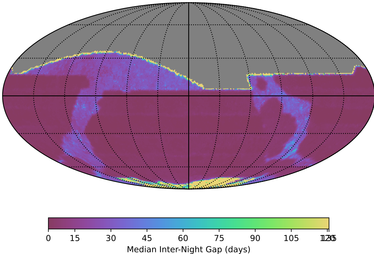
ddf_loaded_fl15_v3.4_10yrs All sky r band: Median Inter-Night Gap
