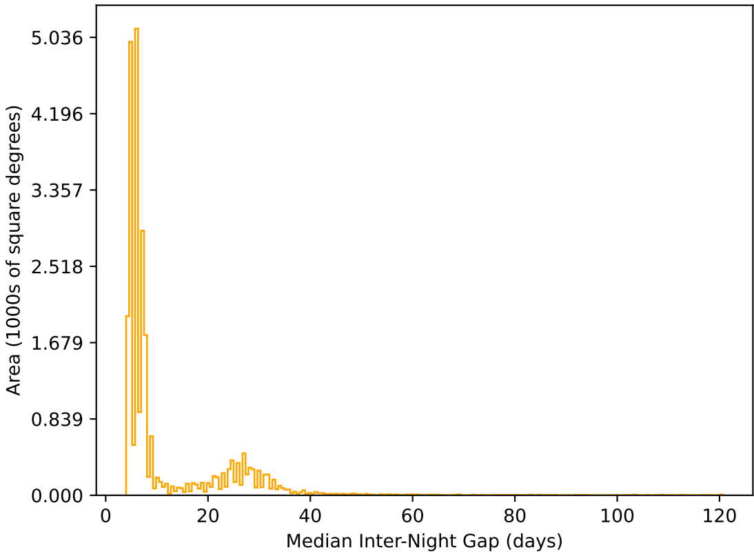
ddf_loaded_fl15_v3.4_10yrs All sky r band: Median Inter-Night Gap
