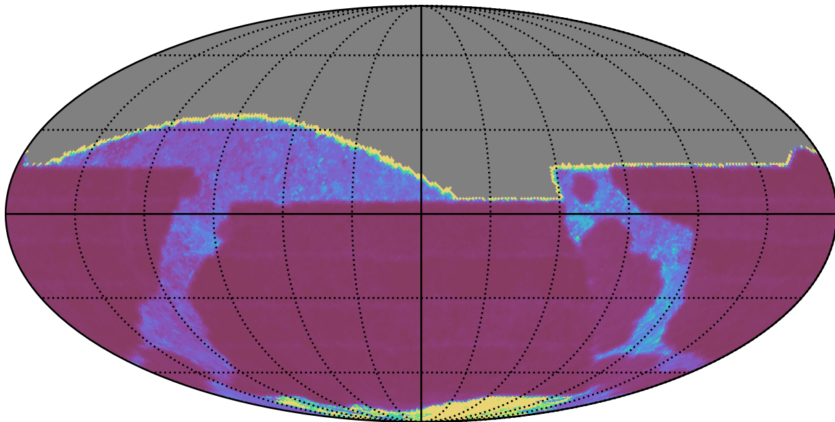
ddf_loaded_fl15_v3.4_10yrs All sky i band: Median Inter-Night Gap
