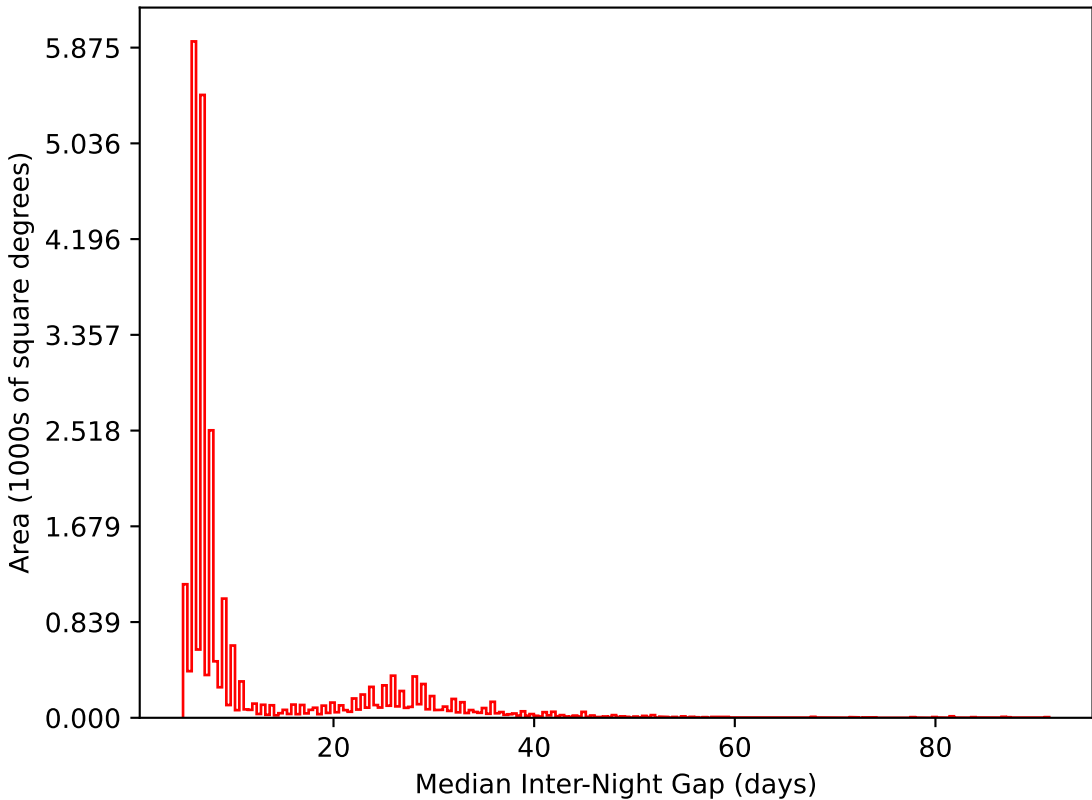
ddf_loaded_fl15_v3.4_10yrs All sky i band: Median Inter-Night Gap
