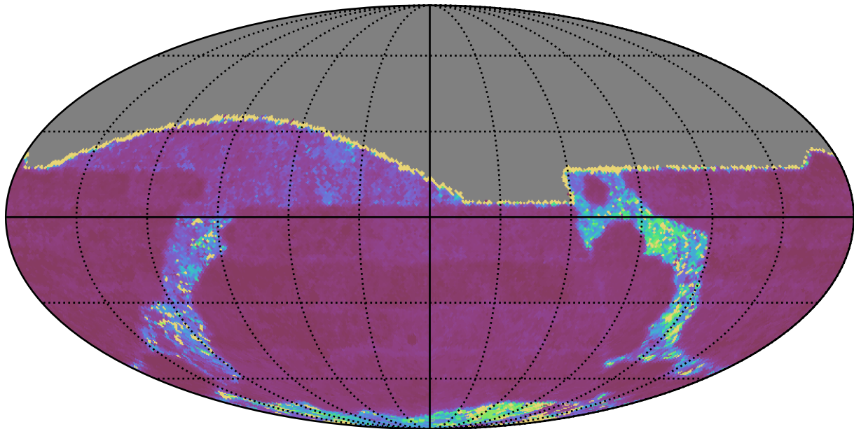
ddf_loaded_fl15_v3.4_10yrs All sky g band: Median Inter-Night Gap
