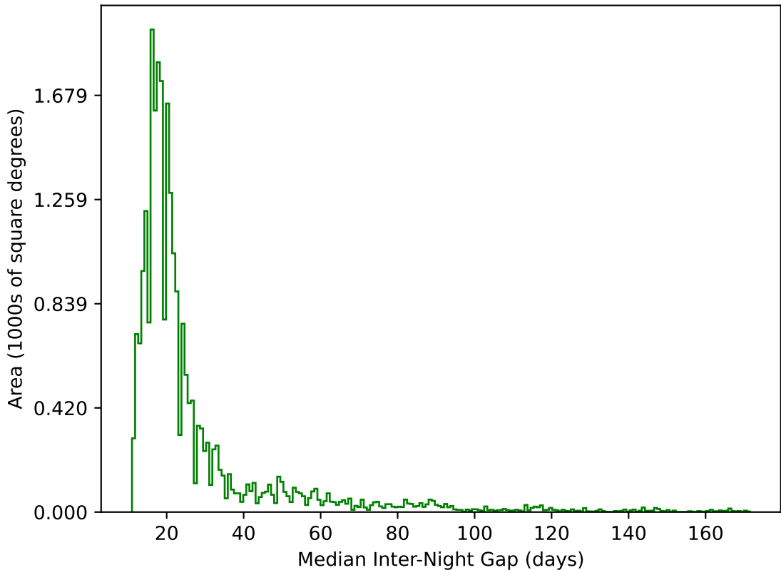
ddf_loaded_fl15_v3.4_10yrs All sky g band: Median Inter-Night Gap
