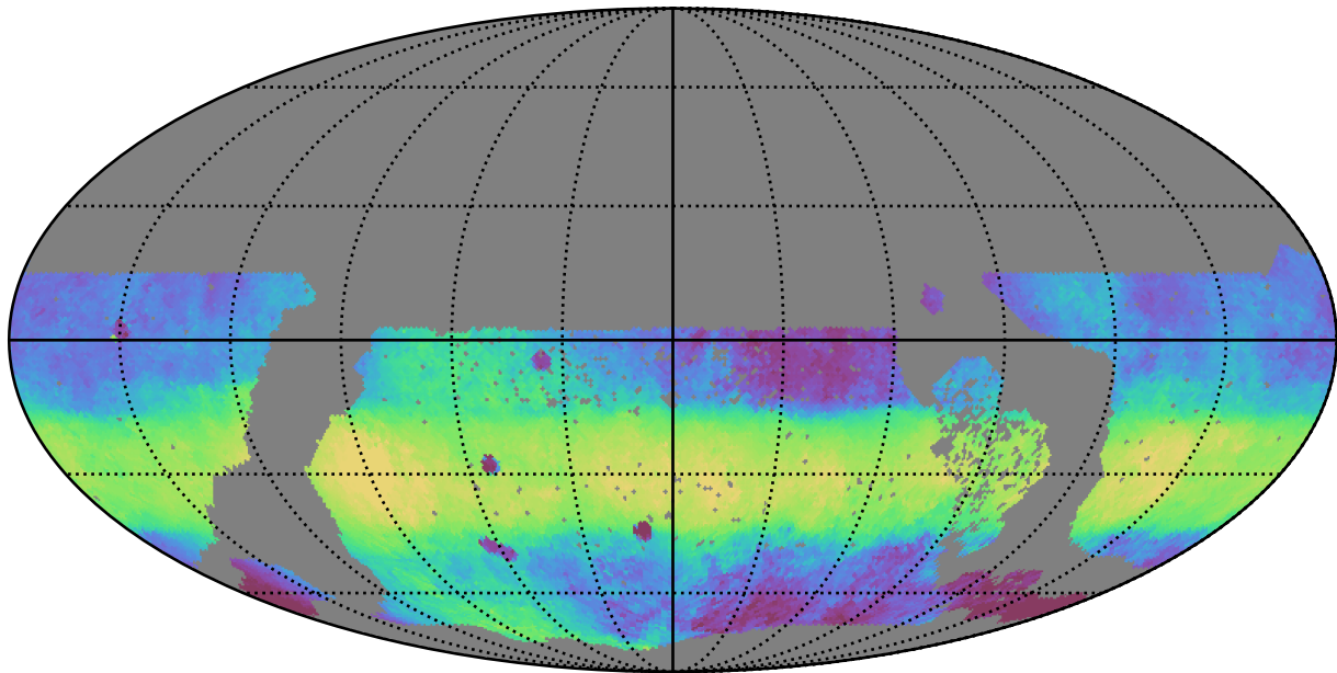
ddf_loaded_fl15_v3.4_10yrs WFD z band: Median HA
