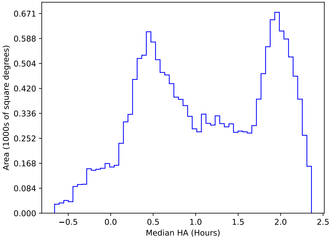
ddf_loaded_fl15_v3.4_10yrs WFD z band: Median HA
