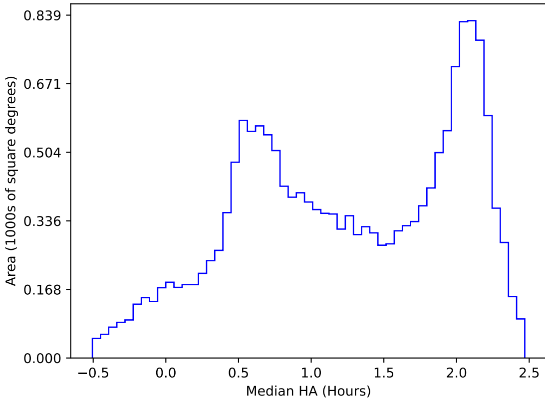
ddf_loaded_fl15_v3.4_10yrs WFD y band: Median HA
