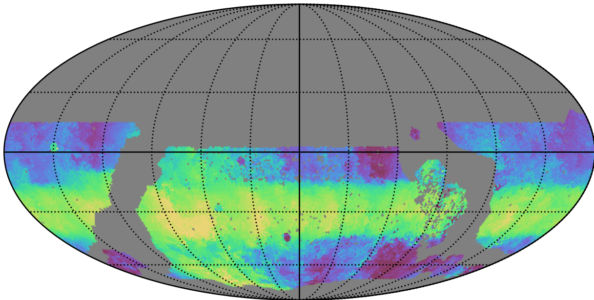
ddf_loaded_fl15_v3.4_10yrs WFD u band: Median HA
