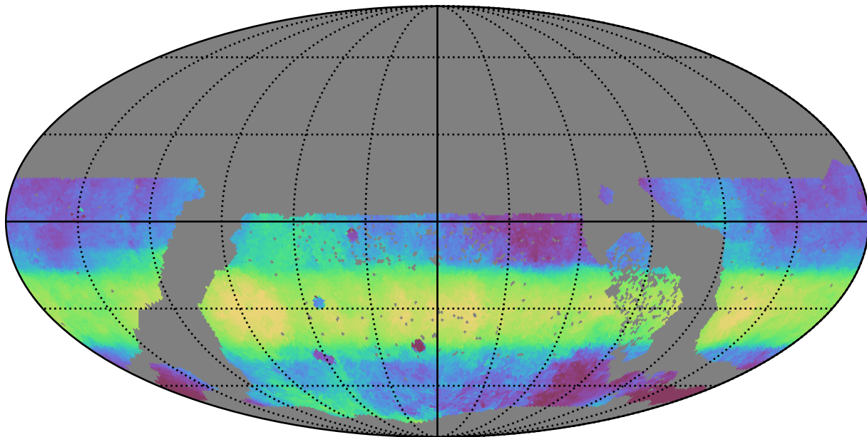
ddf_loaded_fl15_v3.4_10yrs WFD i band: Median HA
