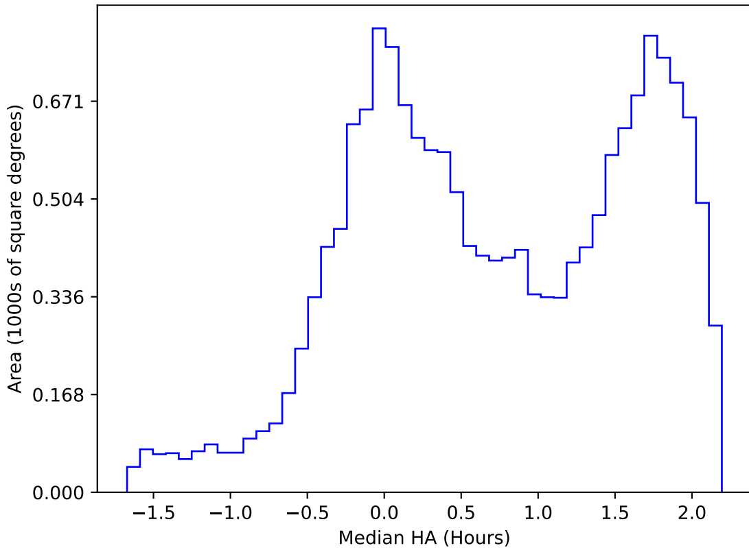
ddf_loaded_fl15_v3.4_10yrs WFD g band: Median HA
