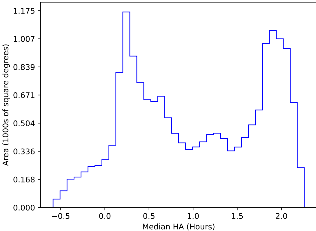
ddf_loaded_fl15_v3.4_10yrs WFD all bands: Median HA
