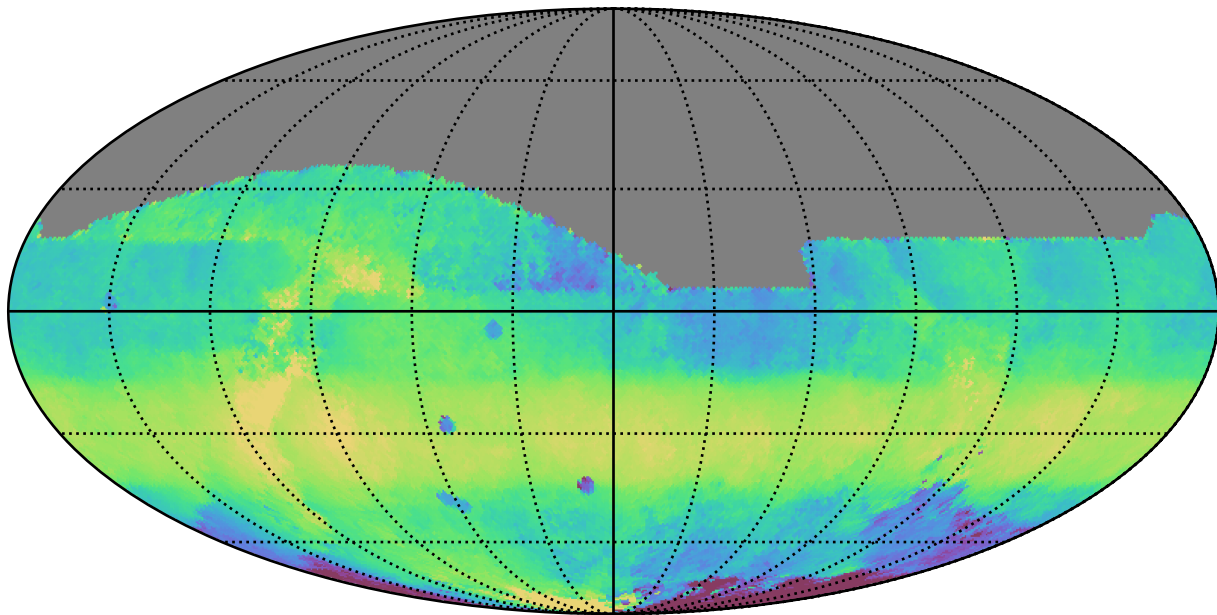
ddf_loaded_fl15_v3.4_10yrs All sky z band: Median HA
