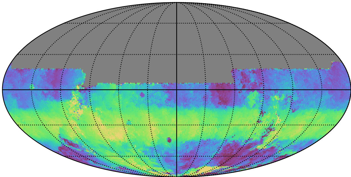
ddf_loaded_fl15_v3.4_10yrs All sky u band: Median HA
