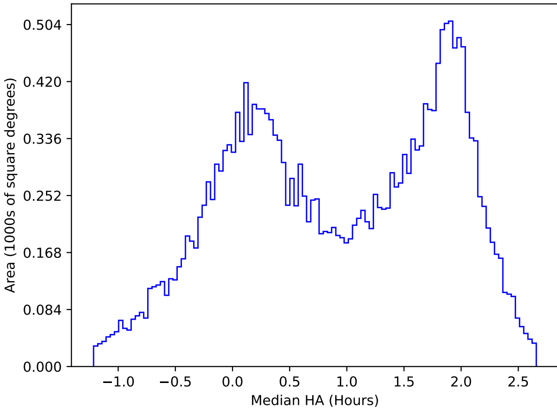
ddf_loaded_fl15_v3.4_10yrs All sky u band: Median HA
