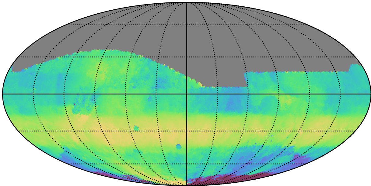
ddf_loaded_fl15_v3.4_10yrs All sky r band: Median HA
