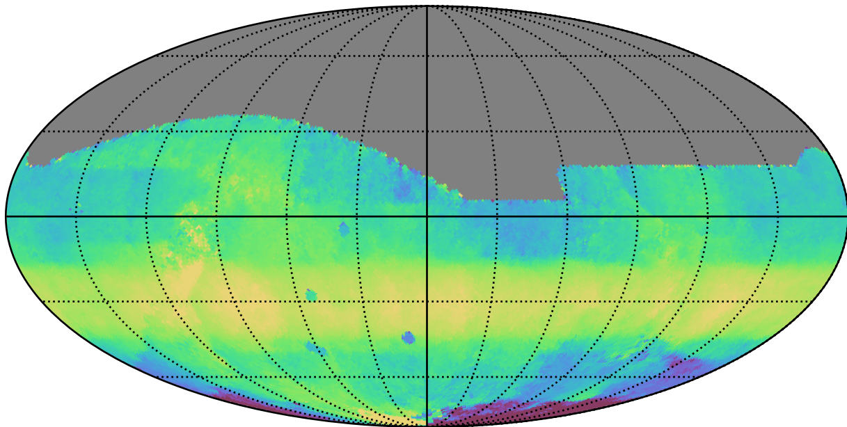
ddf_loaded_fl15_v3.4_10yrs All sky i band: Median HA
