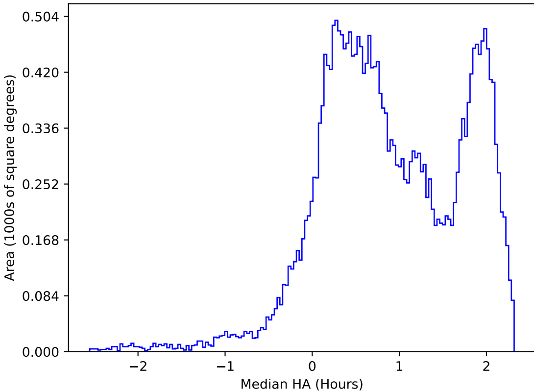
ddf_loaded_fl15_v3.4_10yrs All sky i band: Median HA
