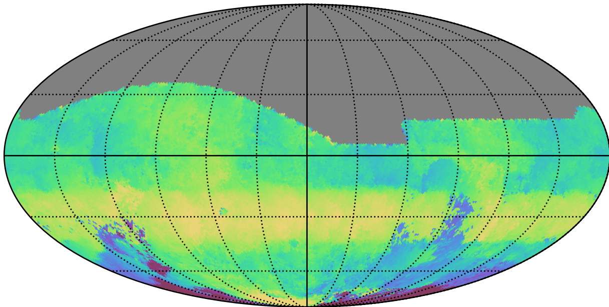
ddf_loaded_fl15_v3.4_10yrs All sky g band: Median HA
