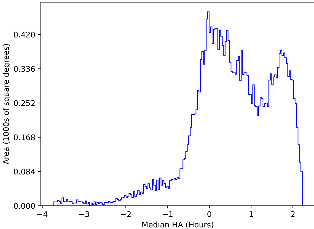
ddf_loaded_fl15_v3.4_10yrs All sky g band: Median HA
