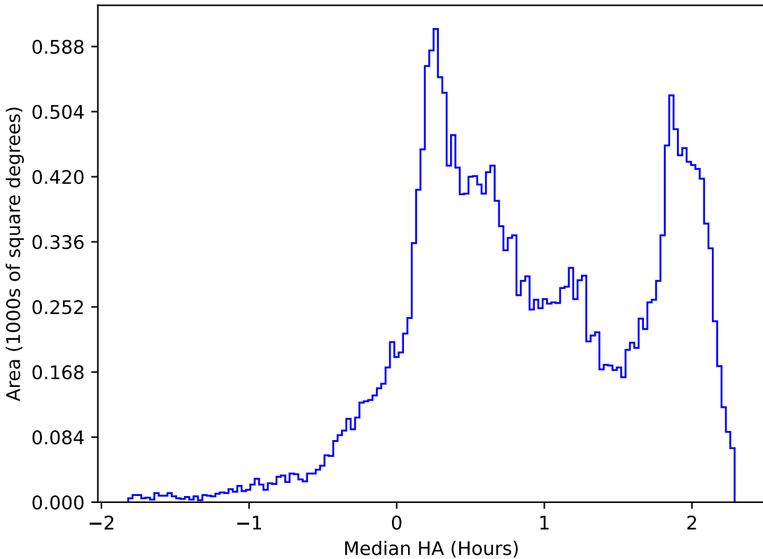
ddf_loaded_fl15_v3.4_10yrs All sky all bands: Median HA
