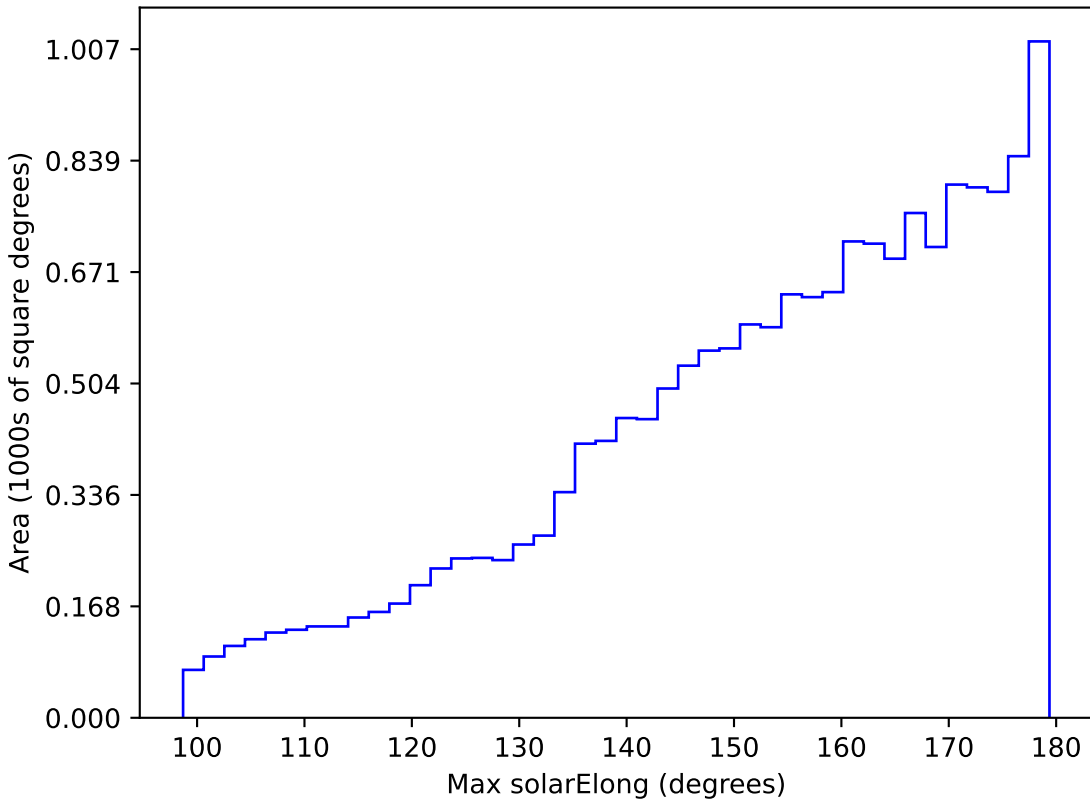
ddf_loaded_fl15_v3.4_10yrs WFD z band: Max solarElong
