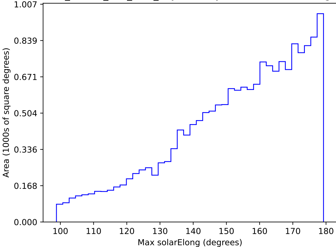
ddf_loaded_fl15_v3.4_10yrs WFD y band: Max solarElong
