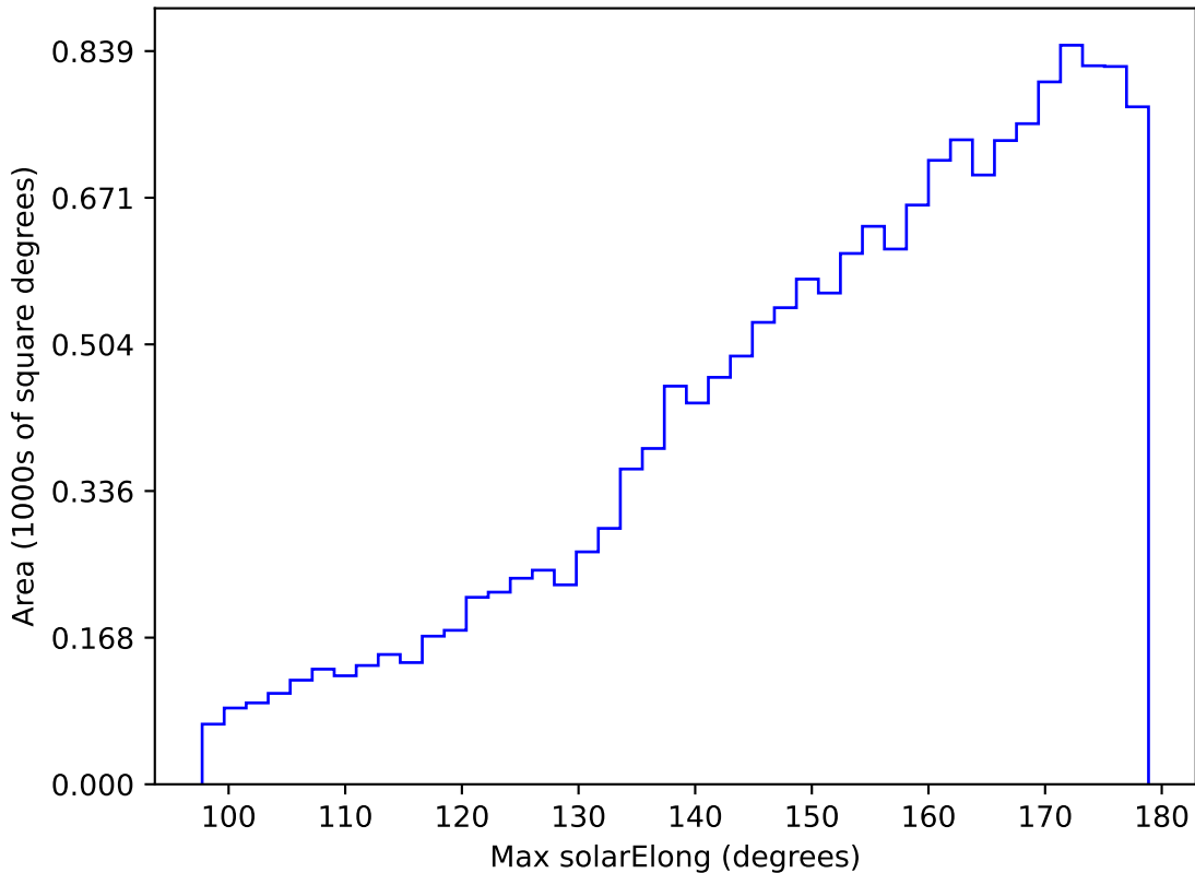
ddf_loaded_fl15_v3.4_10yrs WFD u band: Max solarElong
