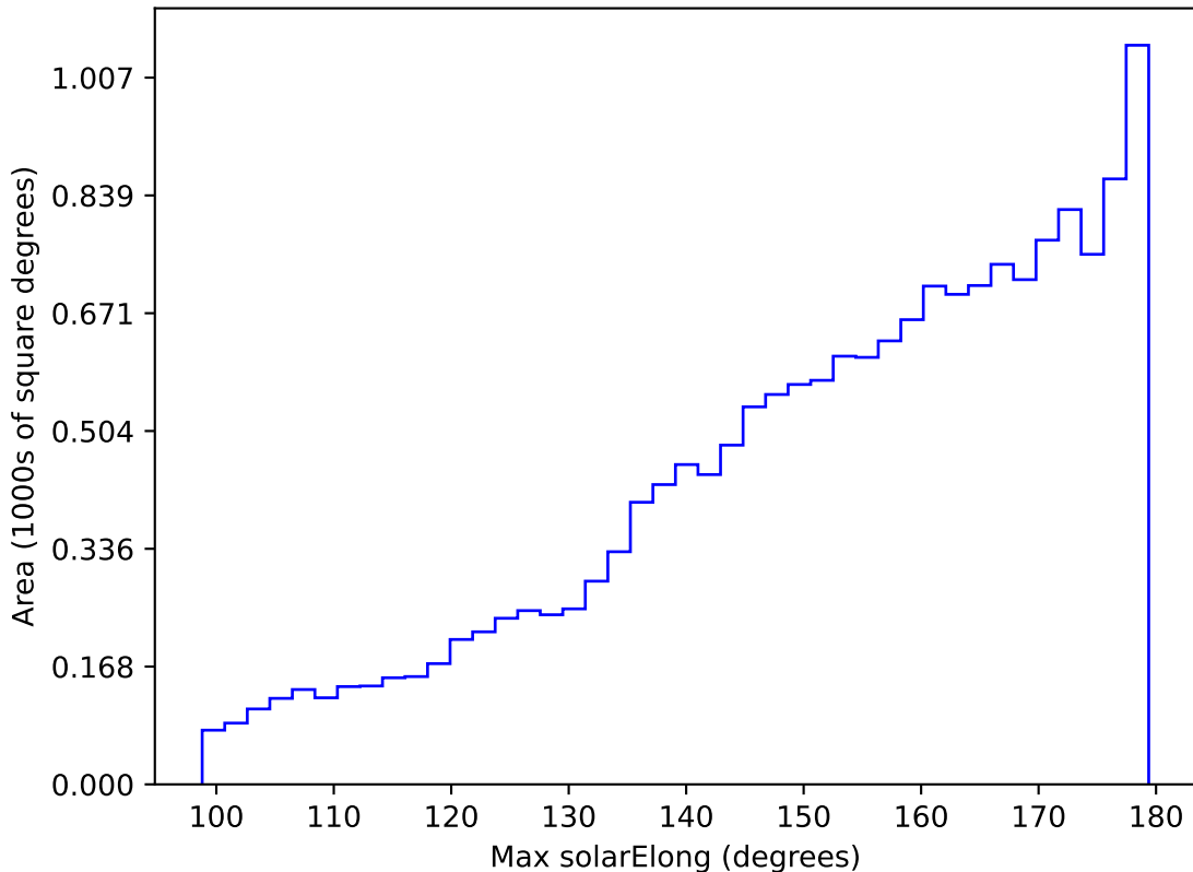
ddf_loaded_fl15_v3.4_10yrs WFD i band: Max solarElong
