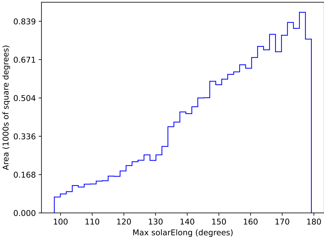
ddf_loaded_fl15_v3.4_10yrs WFD g band: Max solarElong
