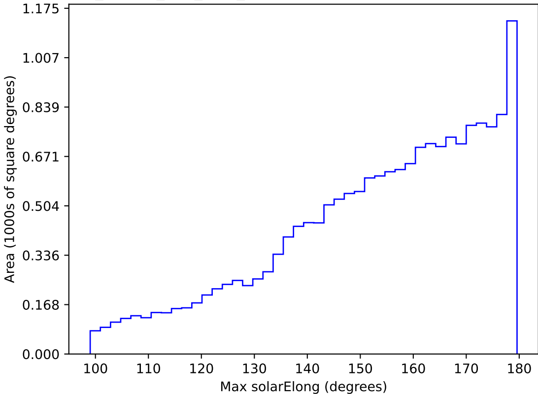
ddf_loaded_fl15_v3.4_10yrs WFD all bands: Max solarElong
