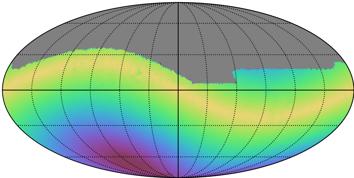
ddf_loaded_fl15_v3.4_10yrs All sky z band: Max solarElong
