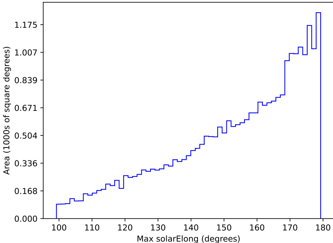
ddf_loaded_fl15_v3.4_10yrs All sky z band: Max solarElong
