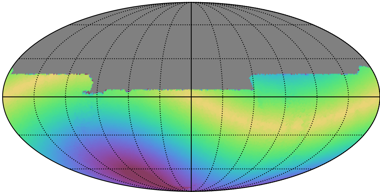
ddf_loaded_fl15_v3.4_10yrs All sky y band: Max solarElong
