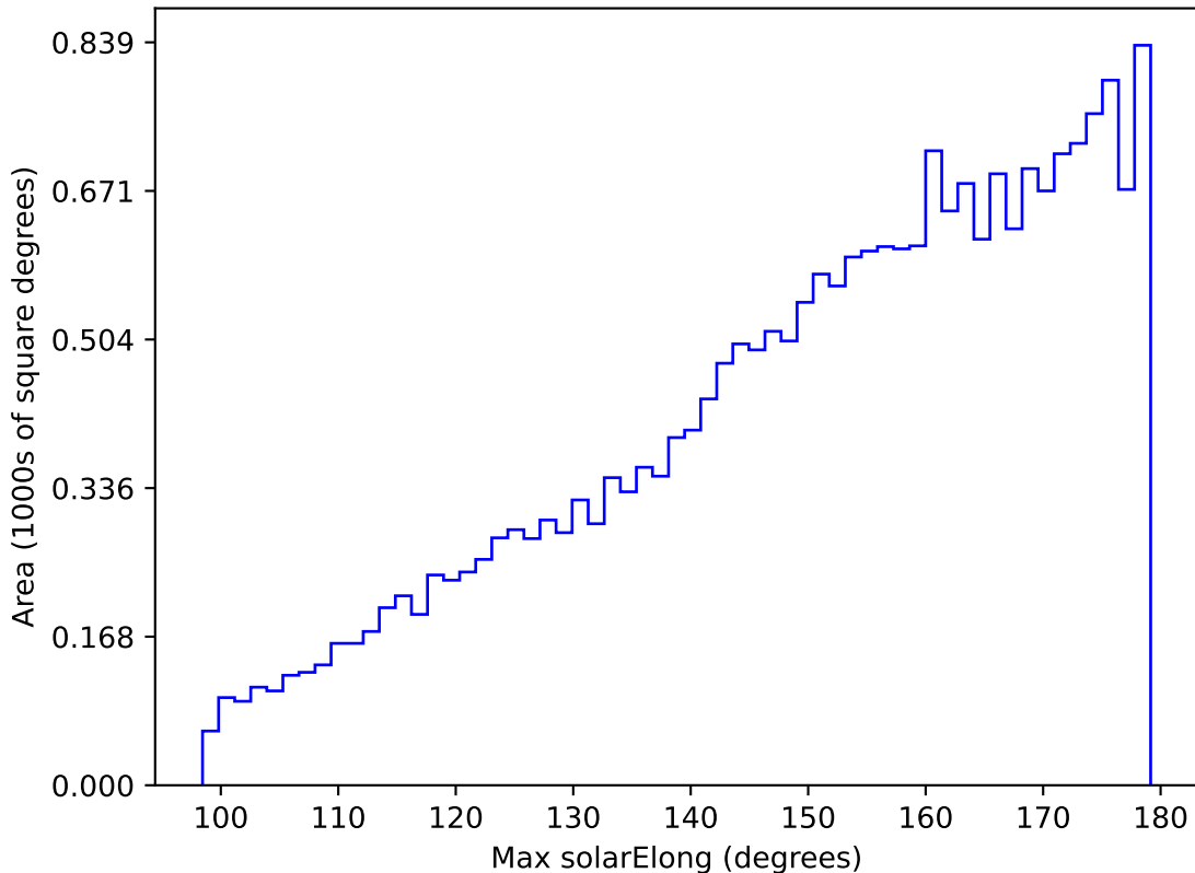
ddf_loaded_fl15_v3.4_10yrs All sky y band: Max solarElong
