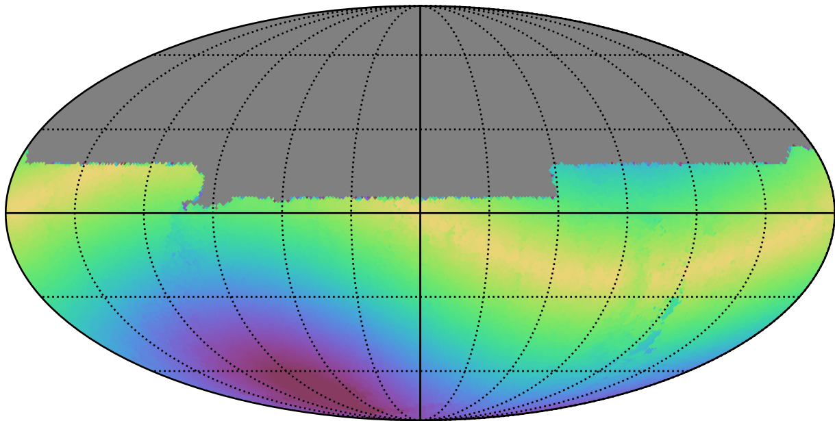
ddf_loaded_fl15_v3.4_10yrs All sky u band: Max solarElong
