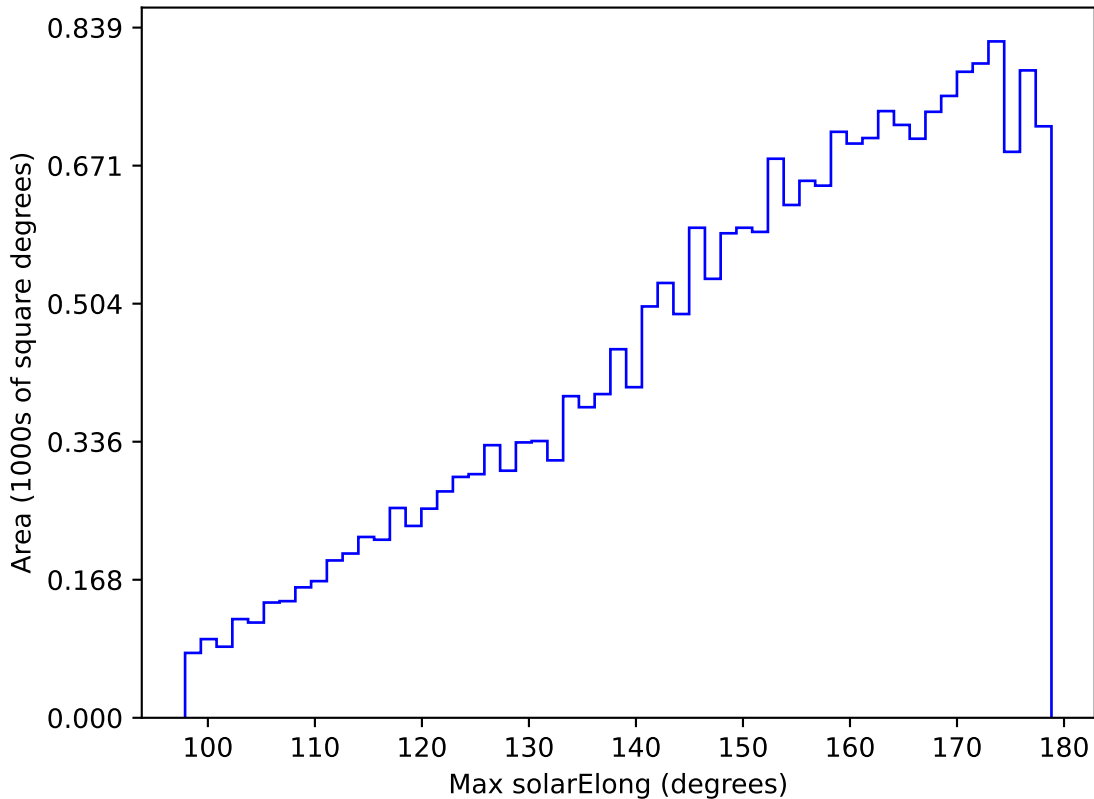
ddf_loaded_fl15_v3.4_10yrs All sky u band: Max solarElong
