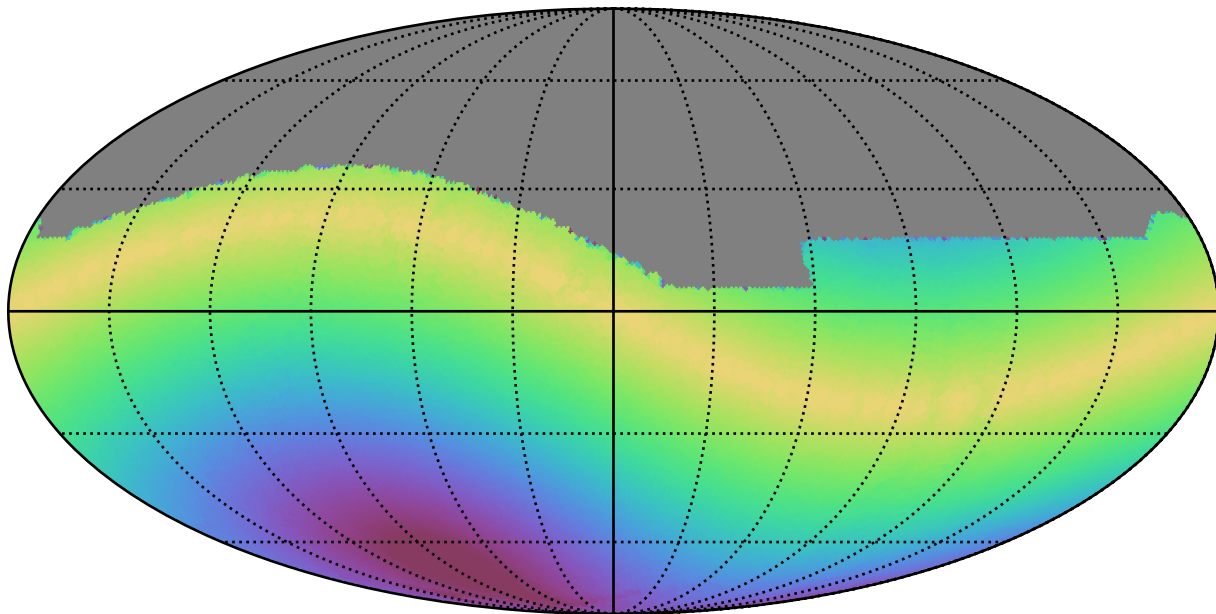
ddf_loaded_fl15_v3.4_10yrs All sky r band: Max solarElong
