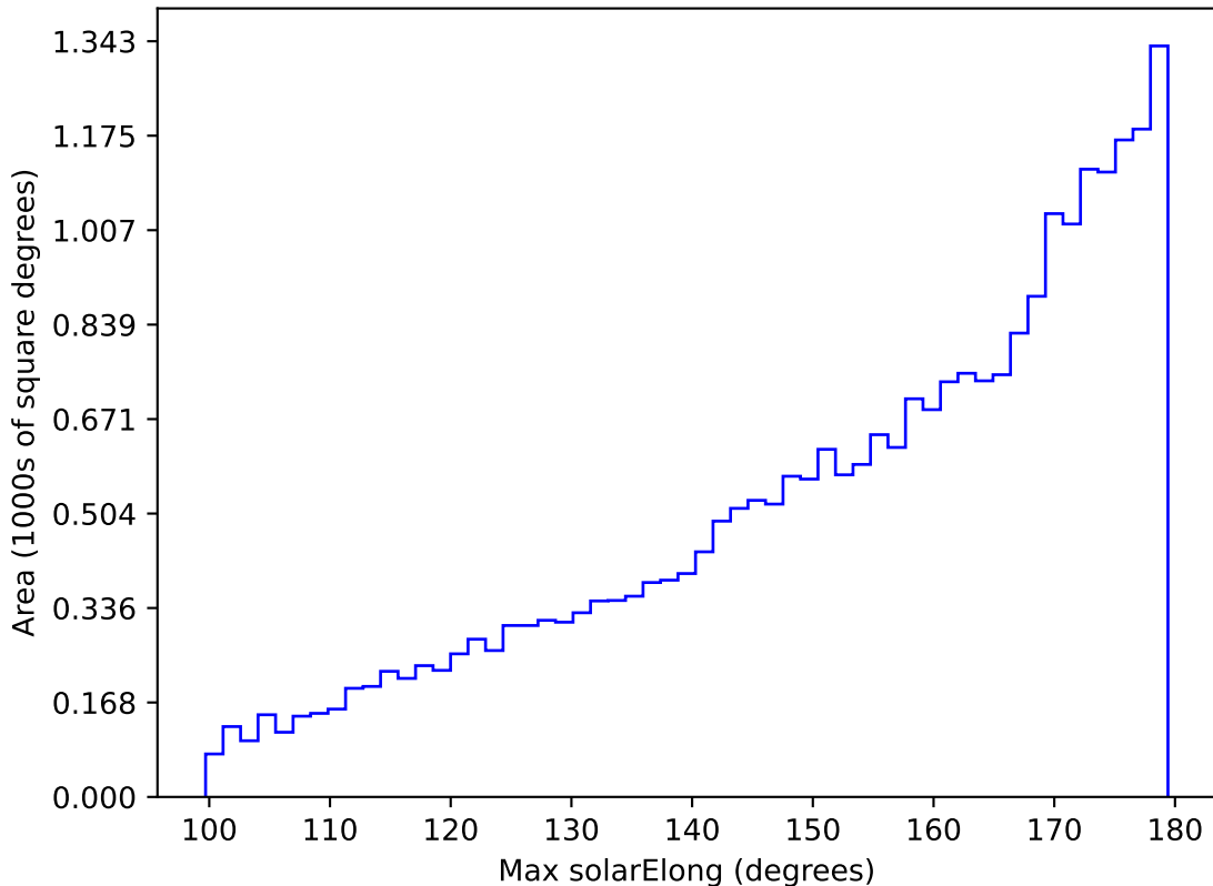
ddf_loaded_fl15_v3.4_10yrs All sky r band: Max solarElong
