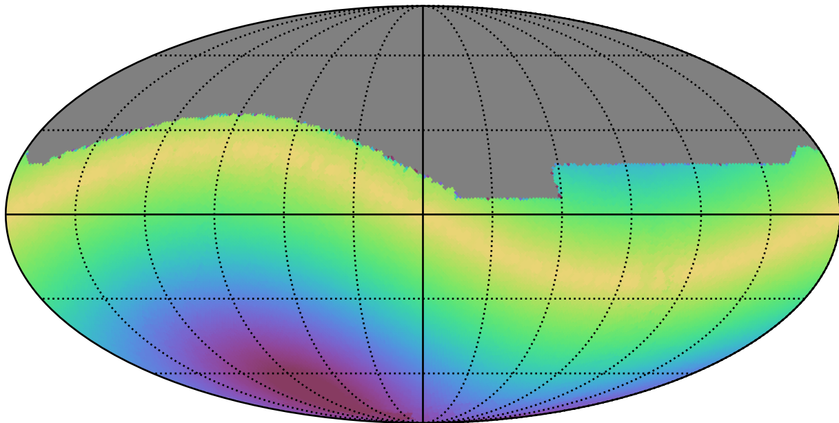
ddf_loaded_fl15_v3.4_10yrs All sky i band: Max solarElong
