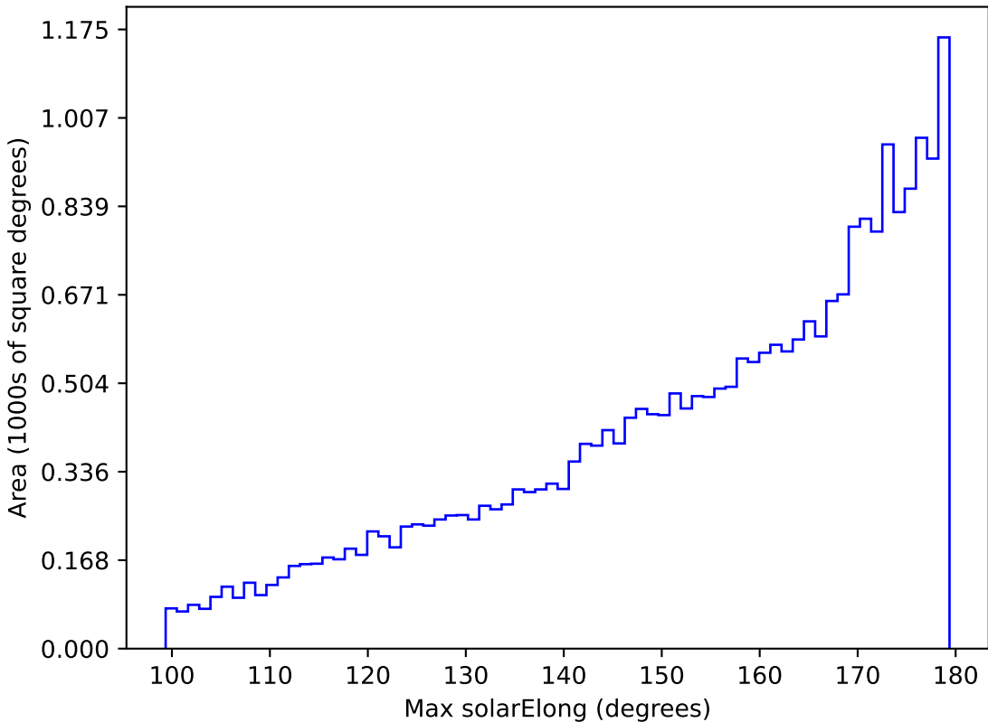
ddf_loaded_fl15_v3.4_10yrs All sky i band: Max solarElong
