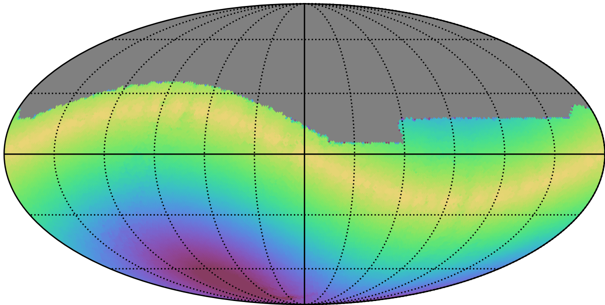
ddf_loaded_fl15_v3.4_10yrs All sky g band: Max solarElong
