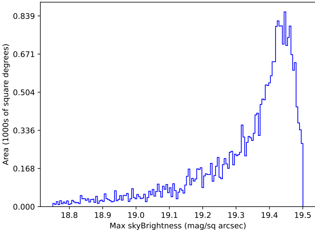
ddf_loaded_fl15_v3.4_10yrs Yr 1 z band: Max skyBrightness
