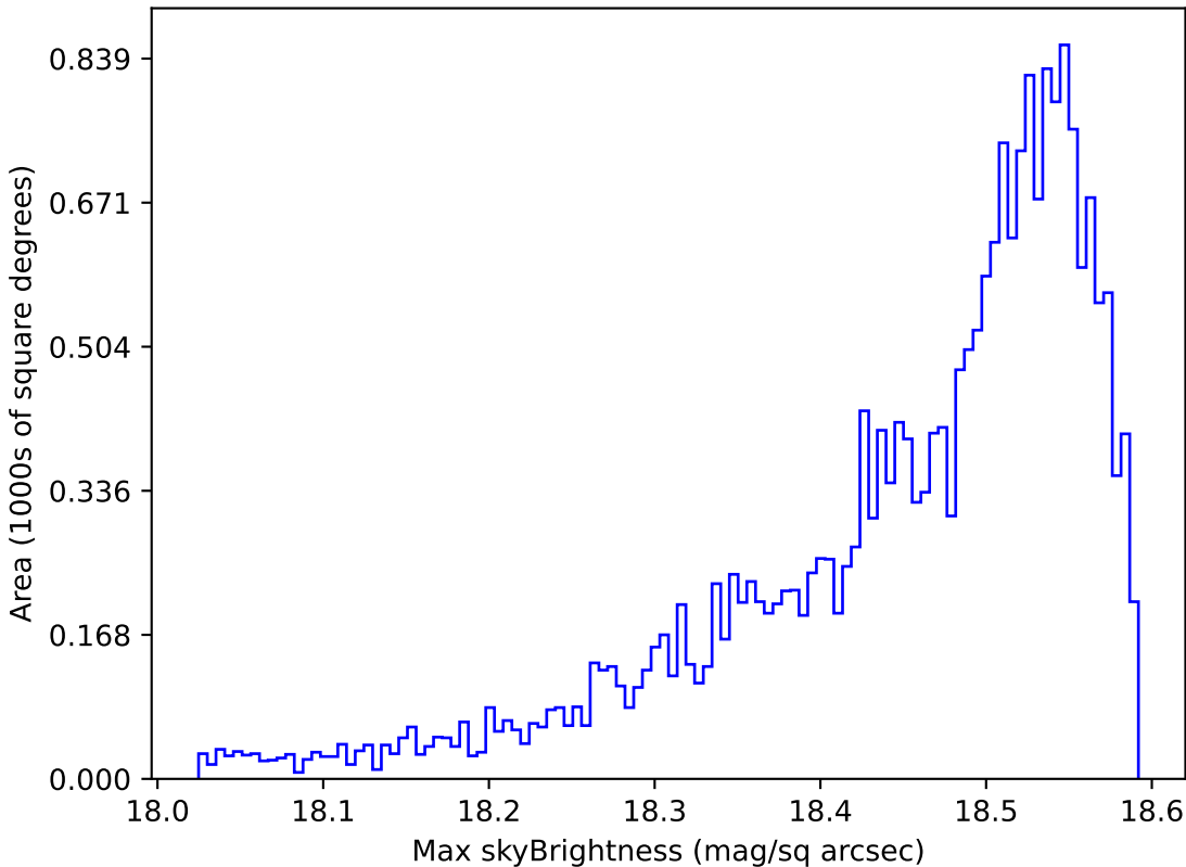
ddf_loaded_fl15_v3.4_10yrs Yr 1 y band: Max skyBrightness
