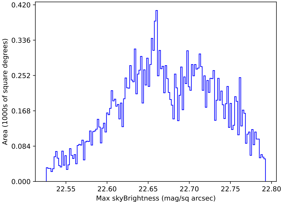
ddf_loaded_fl15_v3.4_10yrs Yr 1 u band: Max skyBrightness
