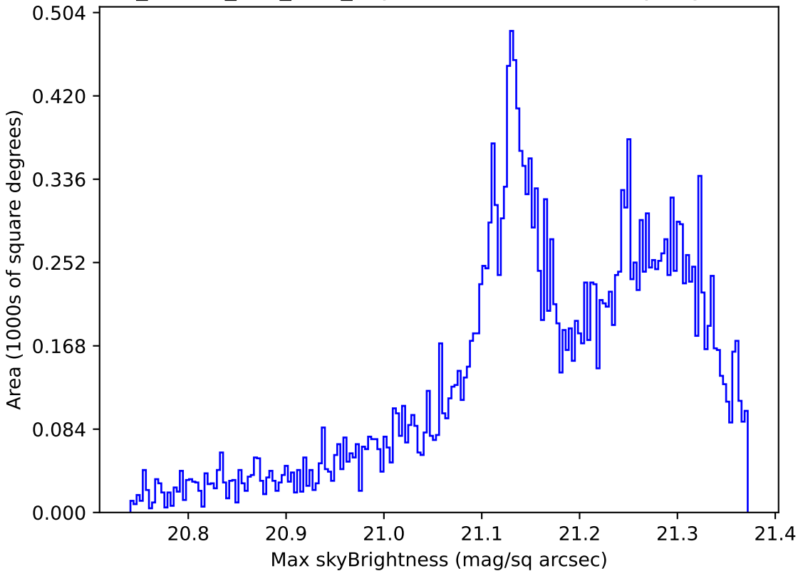
ddf_loaded_fl15_v3.4_10yrs Yr 1 r band: Max skyBrightness
