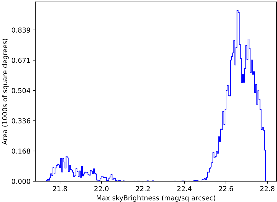
ddf_loaded_fl15_v3.4_10yrs Yr 1 all bands: Max skyBrightness
