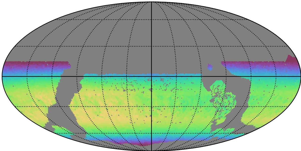
ddf_loaded_fl15_v3.4_10yrs WFD z band: Max skyBrightness
