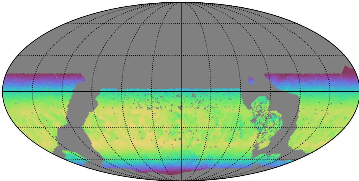
ddf_loaded_fl15_v3.4_10yrs WFD y band: Max skyBrightness
