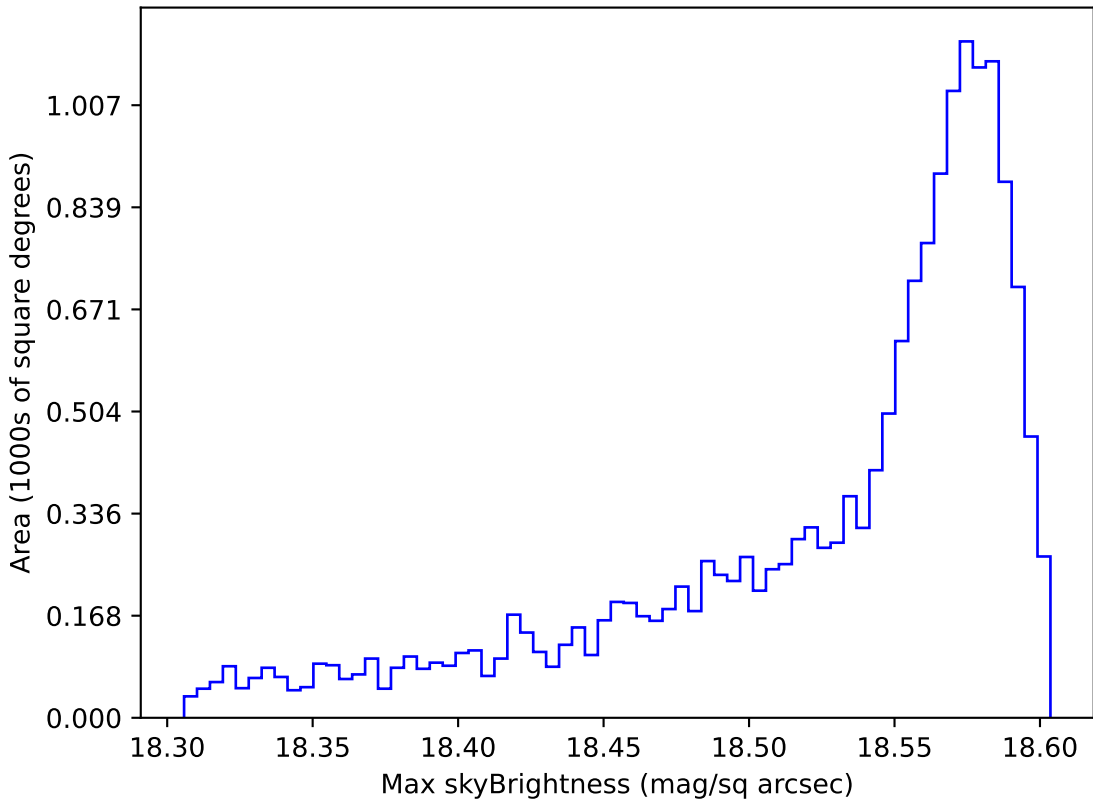
ddf_loaded_fl15_v3.4_10yrs WFD y band: Max skyBrightness
